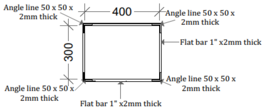
PLAN (Column protection) 12No.
