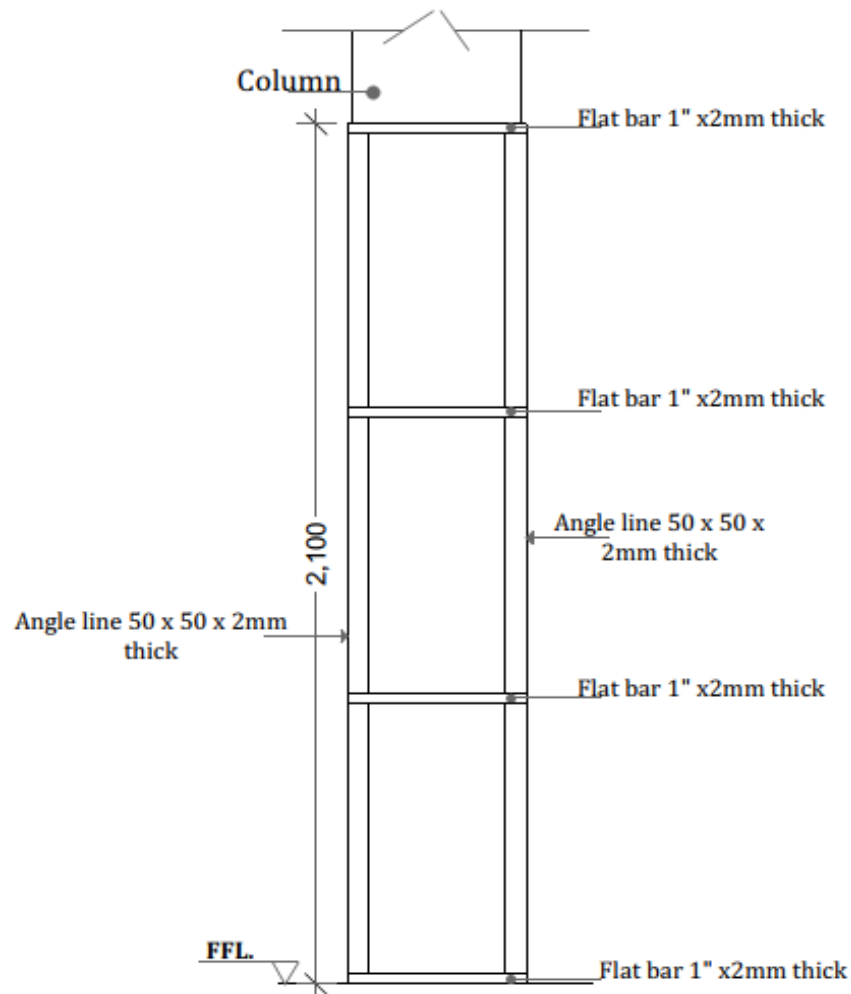
ELEVATION (Column protection)
